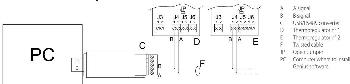
Figure 6.1 Modbus network connection diagram
