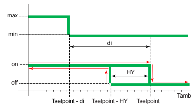
Figure 10.5 Remote independent/assisted mode operation diagram (on/off or modulating)
